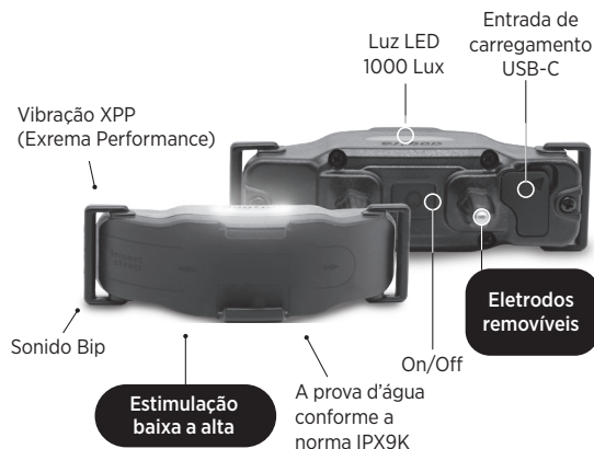
ARC-X Coleira
