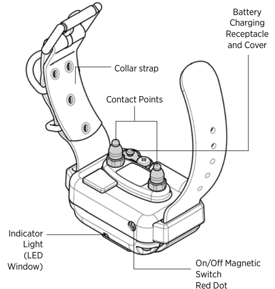
3500NCP Receiver/Collar
