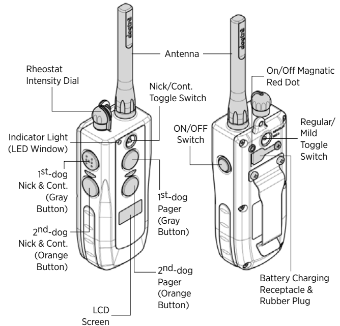
3500NCP Transmitter
