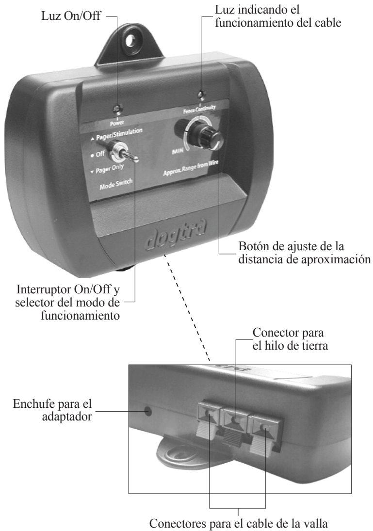
E-FENCE 3500 Transmisor
